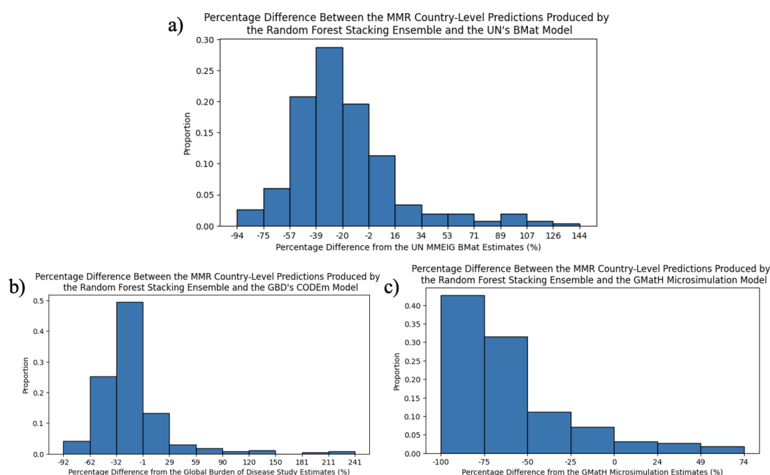
Figure 5.33: Percentage difference between the MMR estimated by my best-performing Random Forest Stacking Ensemble trained for country-level prediction and the MMR estimated by a) BMat, b) CODEm, and c) GMatH.
