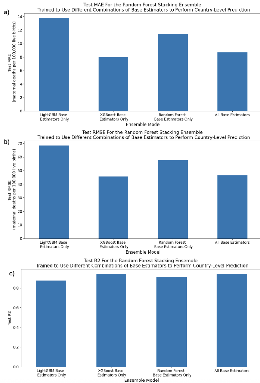
Figure A.13: a) Mean average error, b) root mean-squared error, and c) R^2 for the Random Forest Stacking Ensemble trained to perform country-level prediction using different combinations of base estimators.
