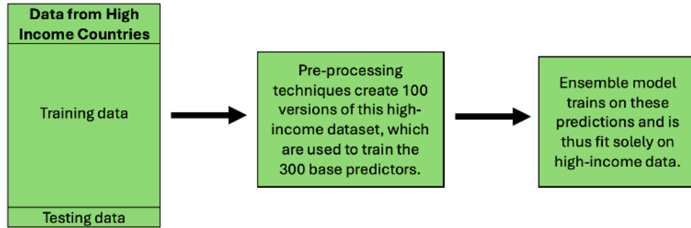
Figure 4.5: Visualisation of the sensitivity analysis procedure, where the ensemble’s base estimators were fit on data from a single income level (in this case, high-income). The sensitivity analysis created a separate ensemble model for each subset of the input data corresponding to a specific income level.
