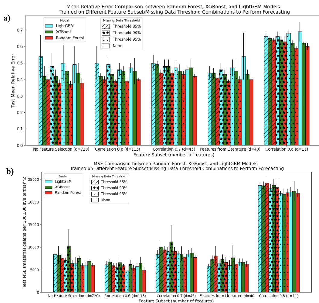
Figure 5.17: a) Mean relative error and b) mean-squared error for Random Forest (red), XGBoost (green), and LightGBM (blue) models fit on different feature subsets and missing data thresholds to perform forecasting.
