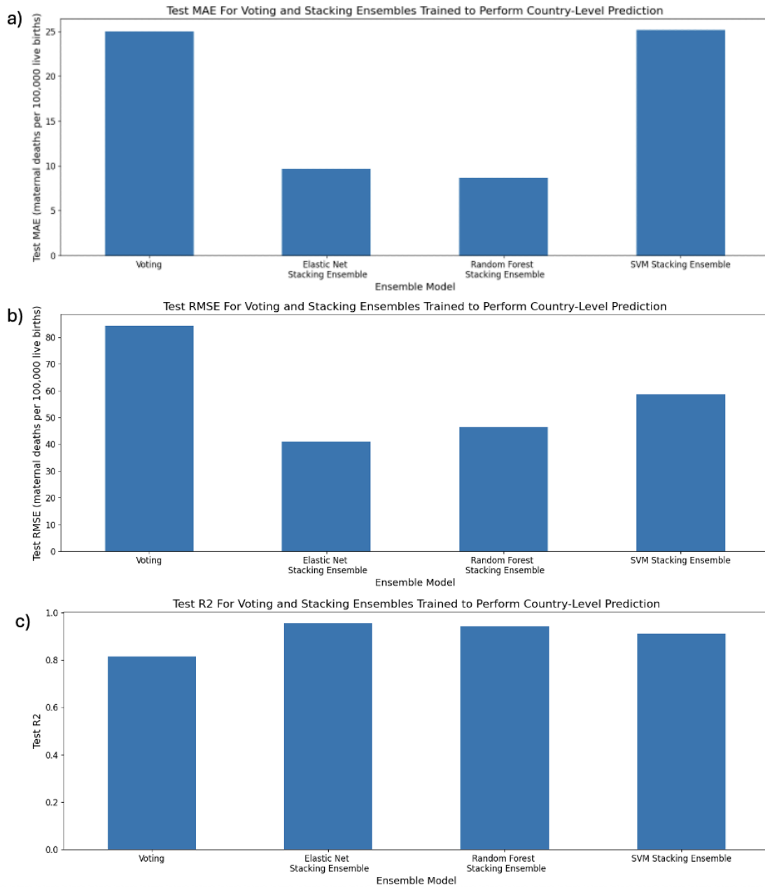
Figure A.9: a) Mean average error, b) root mean-squared error, and c) R^2 for voting and stacking ensembles trained on all base models to perform country-level prediction.
