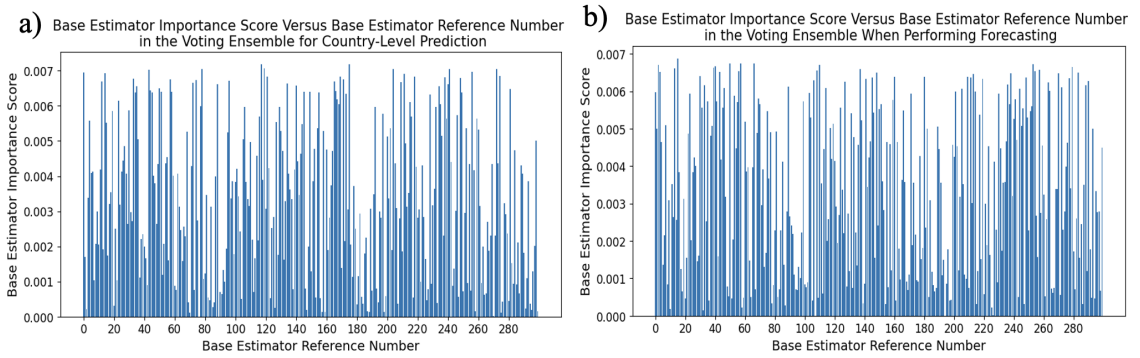
Figure 5.22: Importance score for each of the 300 base estimators used in the Voting Ensemble trained for a) country-level prediction and b) forecasting.
