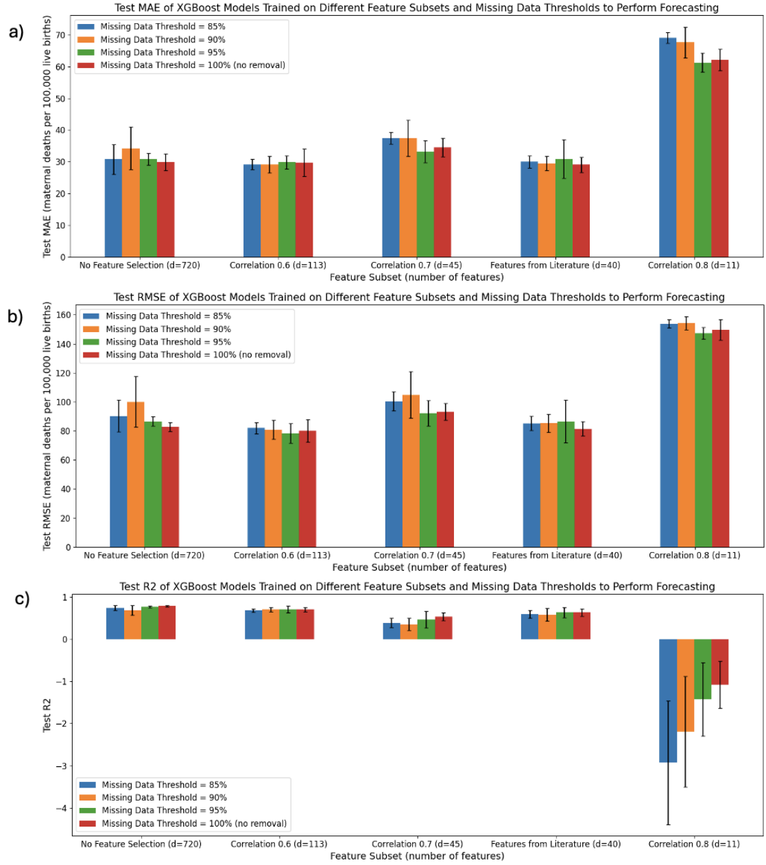
Figure A.5: a) Mean average error, b) root mean-squared error, and c) R^2 for XGBoost base estimators fit on different feature subsets and missing data thresholds to perform forecasting.
