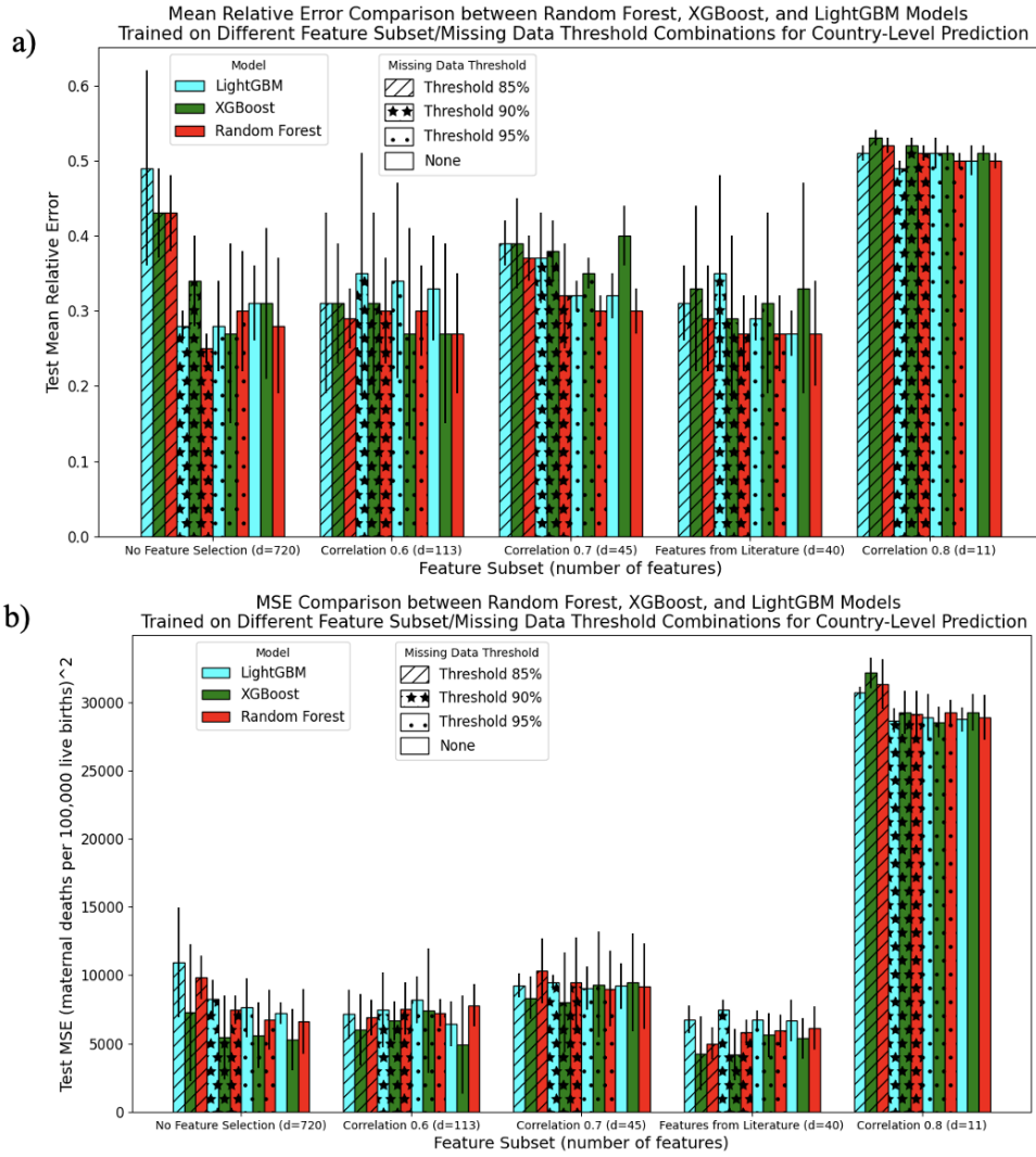
Figure 5.16: a) Mean relative error and b) mean-squared error for Random Forest (red), XGBoost (green), and LightGBM (blue) models fit on different feature subsets and missing data thresholds to perform country-level prediction.
