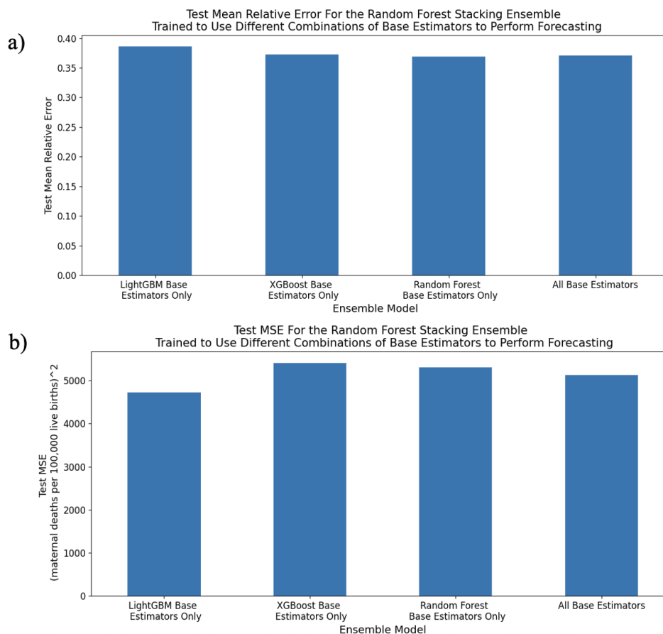
Figure 5.26: a) Mean relative error and b) mean-squared error for the Random Forest Stacking Ensemble trained to perform forecasting using different combinations of base estimators.
