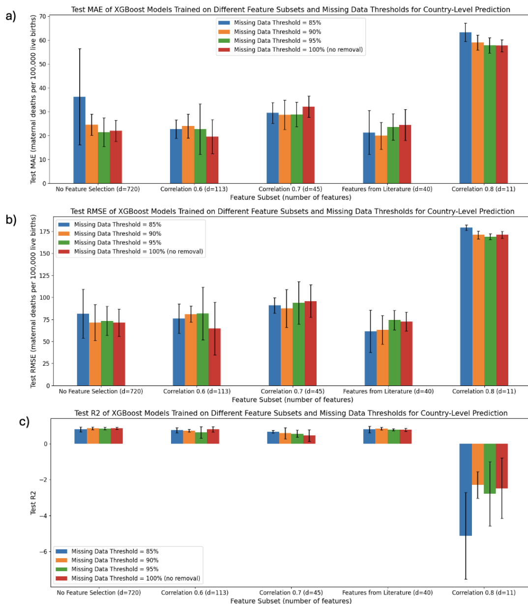
Figure A.2: a) Mean average error, b) root mean-squared error, and c) R^2 for XGBoost base estimators fit on different feature subsets and missing data thresholds for country-level prediction.
