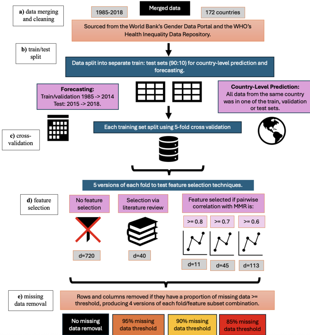
Figure 4.1: High-level overview of the data merging and pre-processing pipeline. I merged data from the WHO and World Bank into a single dataset (a). I then split this data into train/test sets, with separate splits used for country-level prediction and forecasting (b). I further divided each training set into 5 cross-validation folds (c). I then produced 5 versions of each fold using different feature selection methods (d). Finally, I generated 4 versions of each feature subset dataset by removing missing data with different levels of flexibility (e). This process generated 100 versions of the training data.
