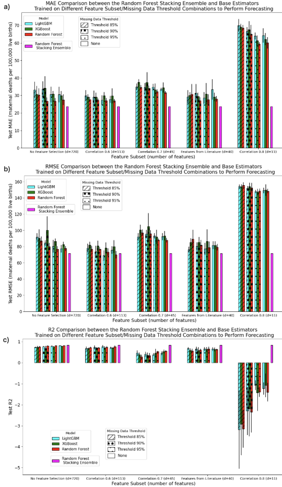
Figure A.12: a) Mean average error, b) root mean-squared error, and c) R^2 for for the Random Forest Stacking Ensemble (purple) and the Random Forest (red), XGBoost (green), and LightGBM (blue) base estimators trained for forecasting.
