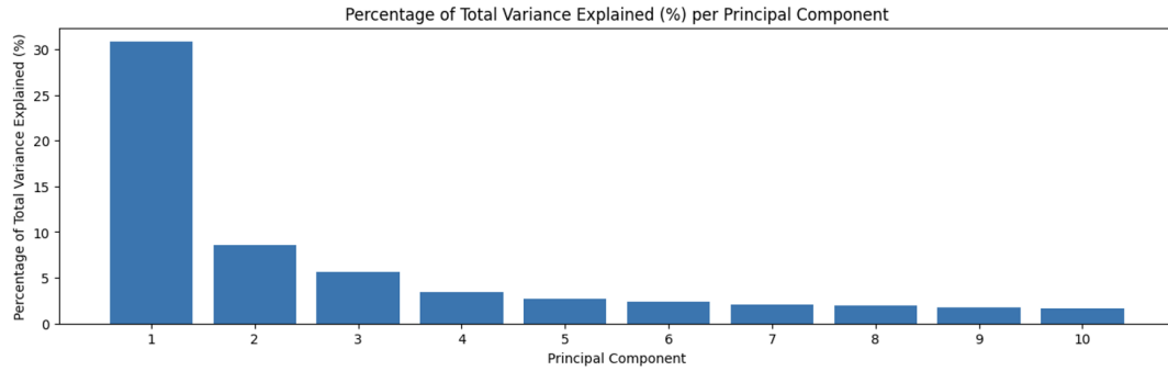
Figure 5.4: Percent of total variance in the dataset captured by the top 10 principal components.
