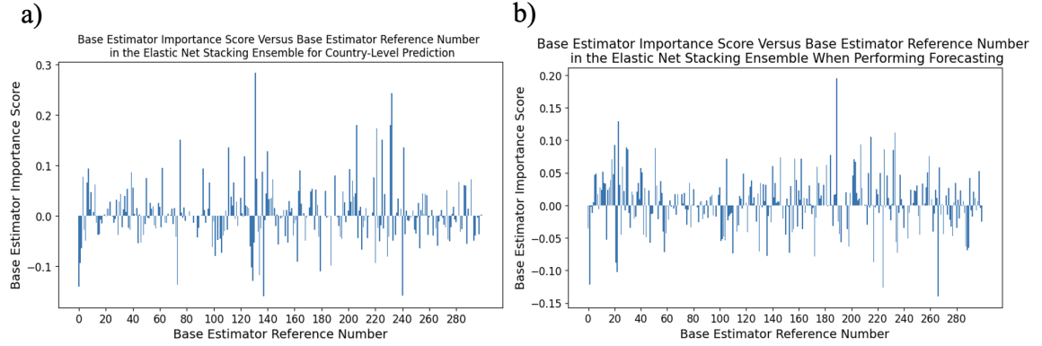
Figure 5.21: Importance score for each of the 300 base estimators used in the Elastic Net Stacking Ensemble trained for a) country-level prediction and b) forecasting.
