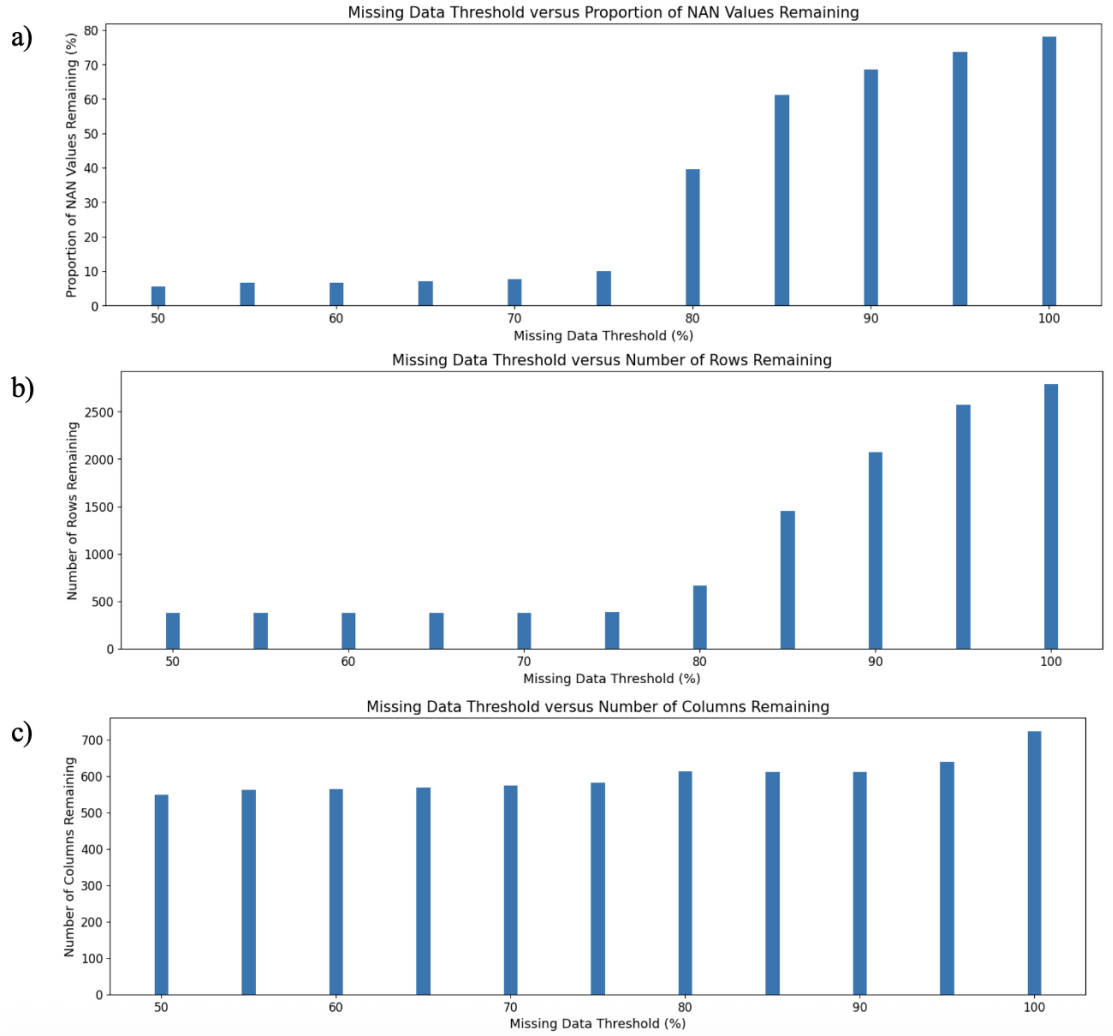
Figure 5.1: The a) proportion of missing data, b) number of rows and c) number of columns remaining in the full input dataset (not split into folds or feature subsets) after missing data removal for thresholds between 50% and 100% (no missing data removed).
