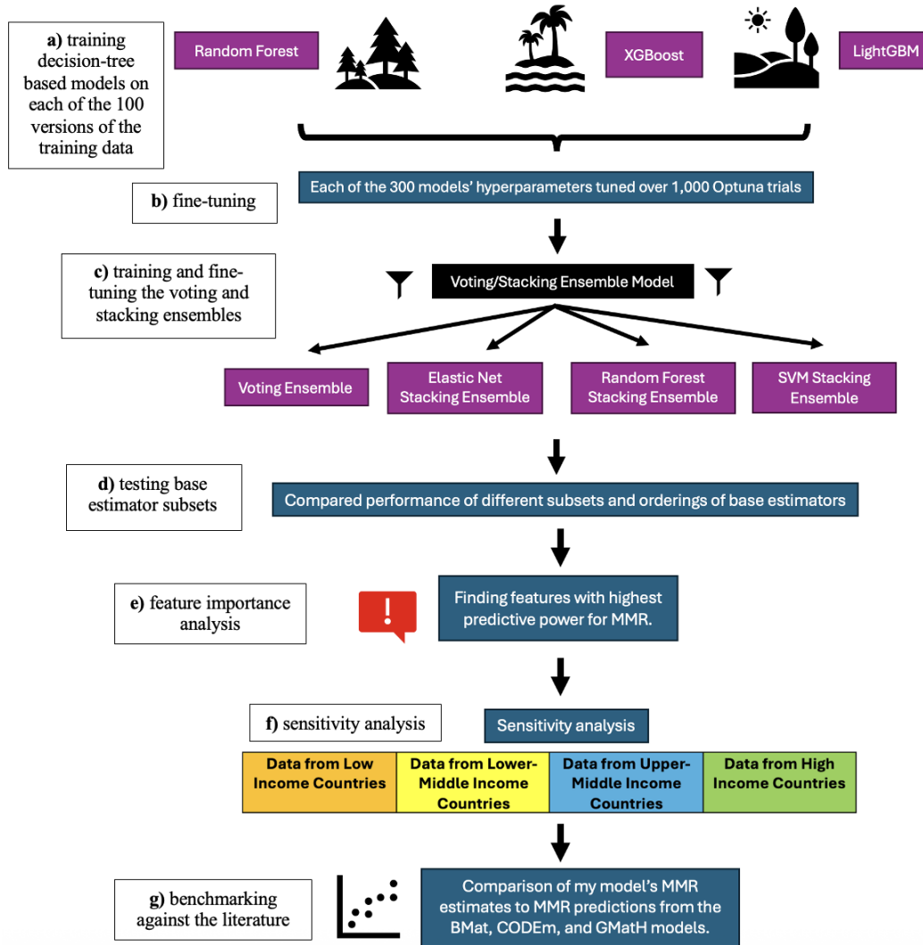
Figure 4.3: Experimental overview of the development of decision-tree based machine learning models used to estimate MMR. Development was done separately for models used to perform country-level prediction and forecasting. Each of the 100 versions the training data was used to fit a single Random Forest, XGBoost, and LightGBM model (a), with each model's hyperparameters fine-tuned over 1000 Optuna trials (b). Different combinations of predictions from each of these base estimators were used to train voting and stacking ensembles (c, d). The features with the highest predictive power for MMR in the best-performing model were identified (e). Finally, the best-performing model's sensitivity to the input data and similarity to MMR predictions from existing models was tested (f, g).
