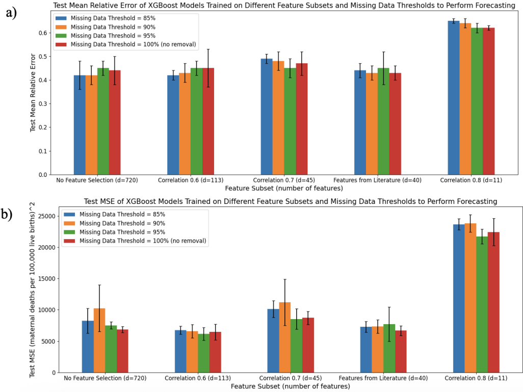
Figure 5.14: a) Mean relative error and b) mean-squared error for XGBoost base estimators fit on different feature subsets and missing data thresholds for forecasting.
