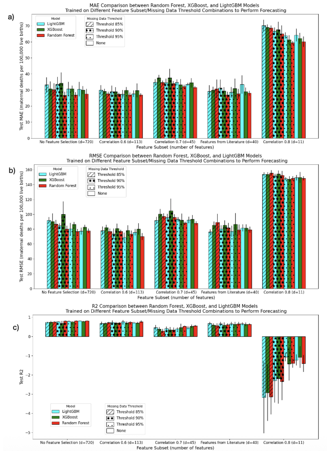
Figure A.8: a) Mean average error, b) root mean-squared error, and c) R^2 for Random Forest (red), XGBoost (green), and LightGBM (blue) models fit on different feature subsets and missing data thresholds to perform forecasting.
