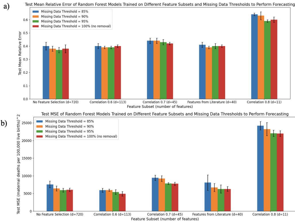
Figure 5.13: a) Mean relative error and b) mean-squared error for Random Forest base estimators fit on different feature subsets and missing data thresholds for forecasting.
