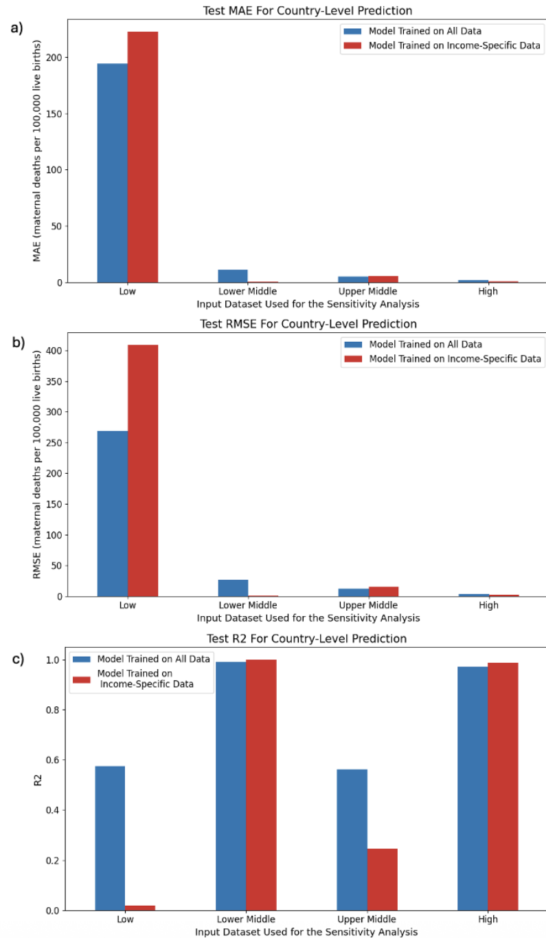
Figure A.15: a) Mean average error, b) root mean-squared error, and c) R^2 for the Random Forest Stacking Ensemble trained on data from all income levels (blue) and RFSEs trained on data from a specific income level (red) to perform country-level prediction. The models being compared were tested on data from the same income level.
