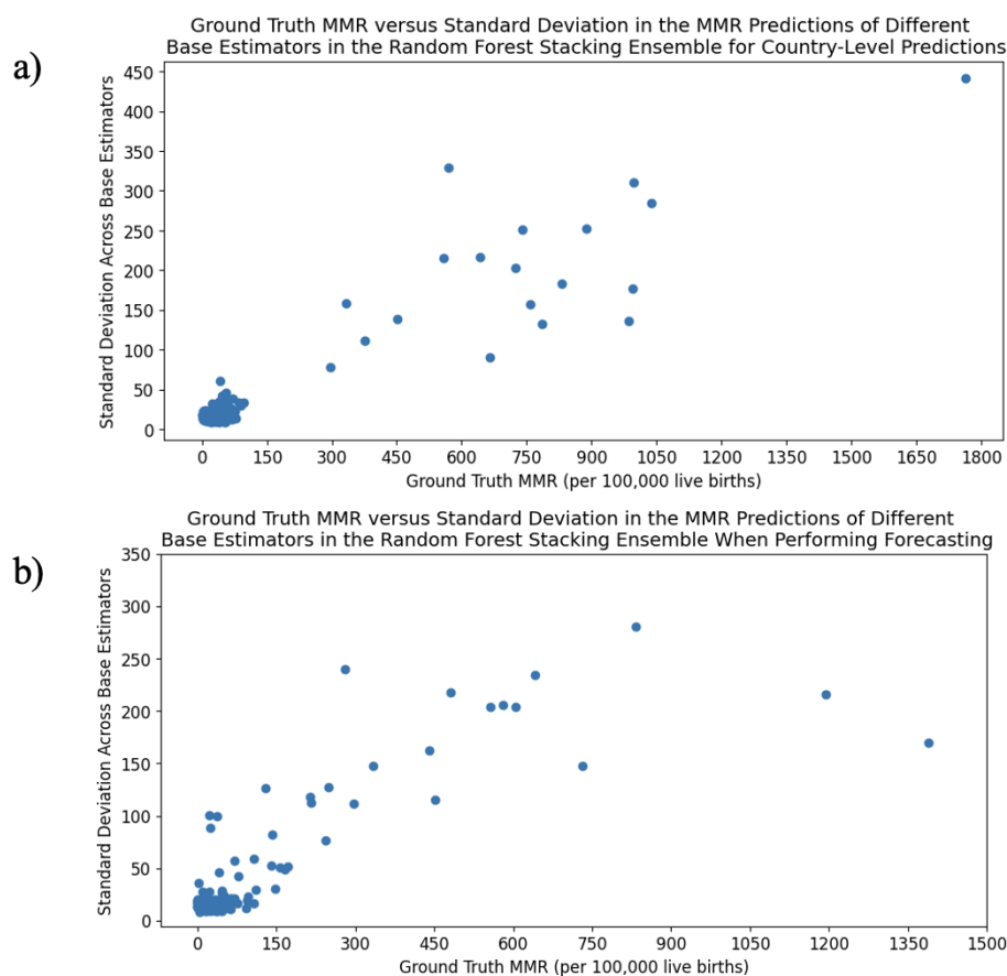
Figure 5.30: Standard deviation among the predictions made by base estimators in the Random Forest Stacking Ensemble versus the ground truth MMR estimate they were trying to predict. This analysis was done for base estimators trained to perform a) country-level prediction and b) forecasting.
