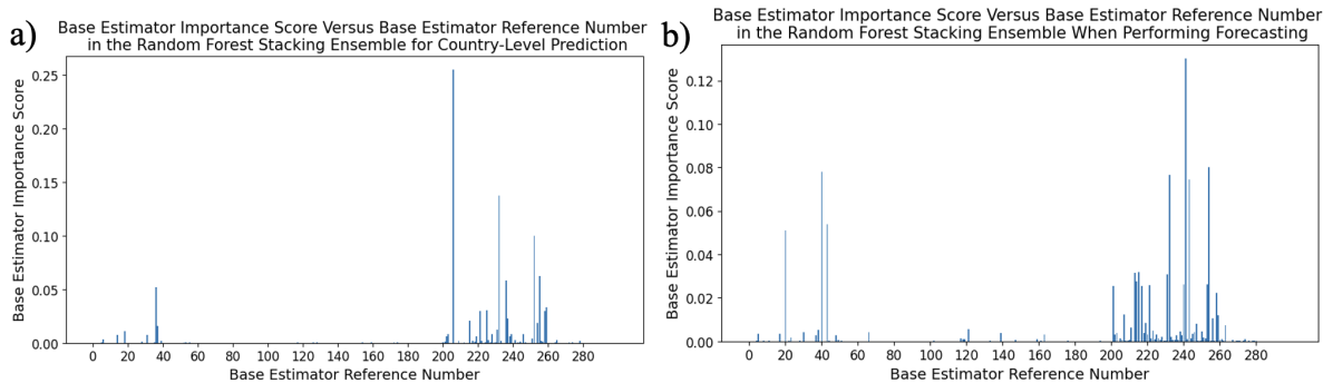
Figure 5.20: Importance score for each of the 300 base estimators used in the Random Forest Stacking Ensemble trained for a) country-level prediction and b) forecasting.
