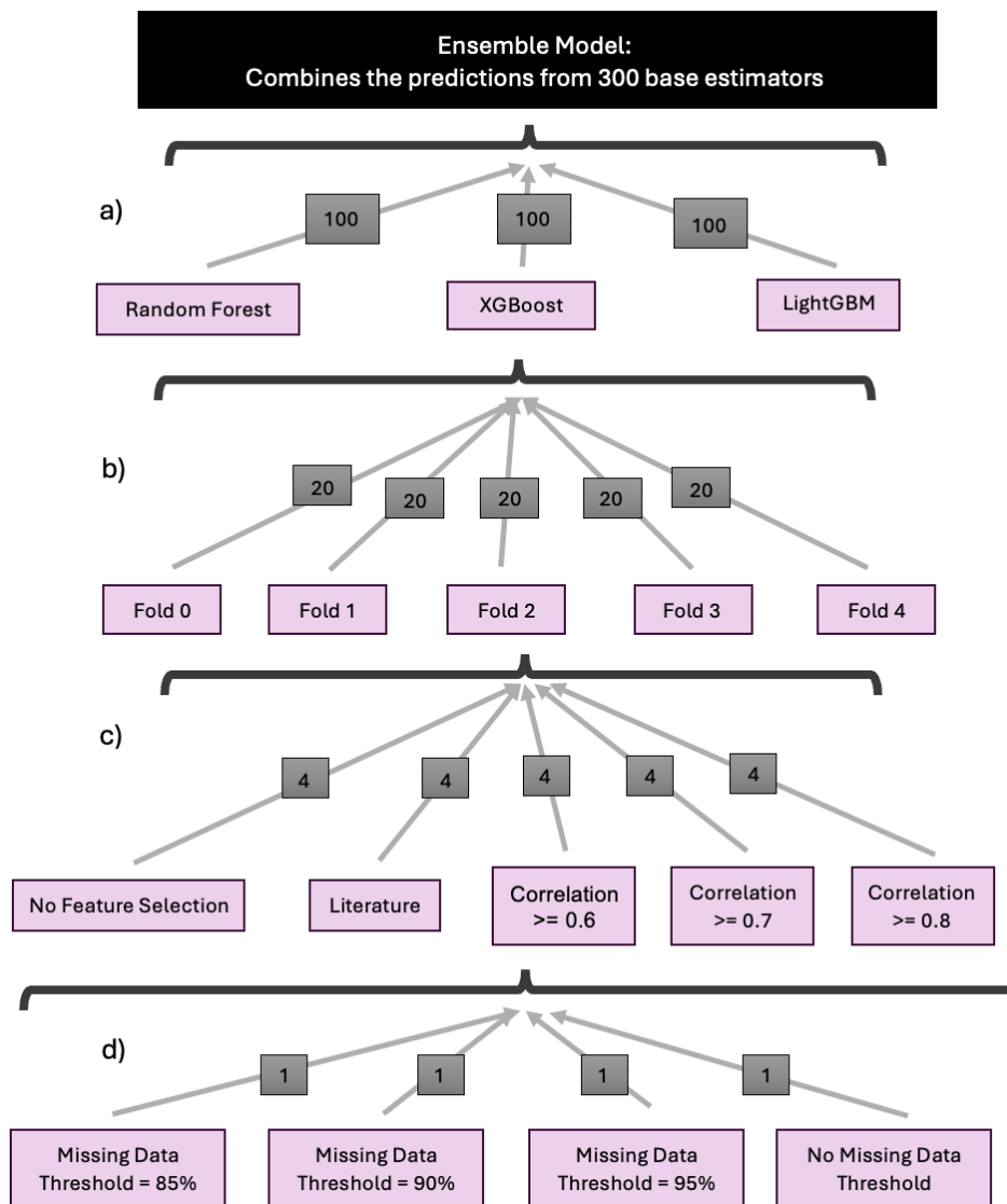
Figure 4.4: Visualisation of the source of the 300 base estimators used as input into the ensemble models. The grey boxes gave the number of base estimators trained per method. The 300 base estimators consisted of 100 Random Forest, XGBoost, and LightGBM models (a). 20 versions of each model-type were trained on each cross-validation fold (b), with the 4 models from the same fold trained on different feature subsets (c). Each of these 4 models were trained on a dataset with a different missing data threshold (d).
