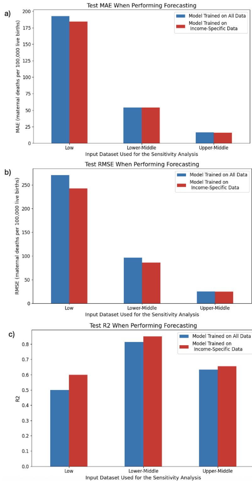
Figure A.16: a) Mean average error, b) root mean-squared error, and c) R^2 for the Random Forest Stacking Ensemble trained on data from all income levels (blue) and RFSEs trained on data from a specific income level (red) to perform forecasting. The models being compared were tested on data from the same income level.
