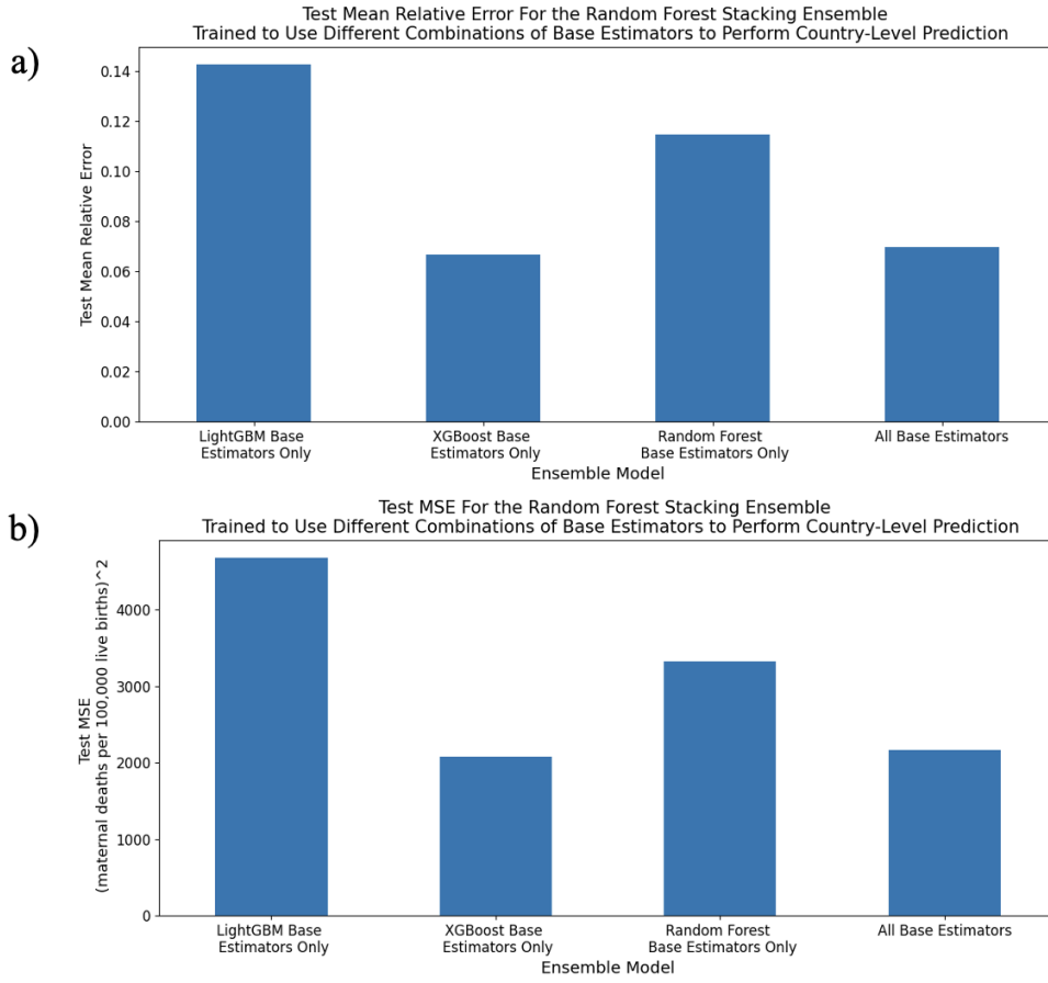
Figure 5.25: a) Mean relative error and b) mean-squared error for the Random Forest Stacking Ensemble trained to perform country-level prediction using different combinations of base estimators.
