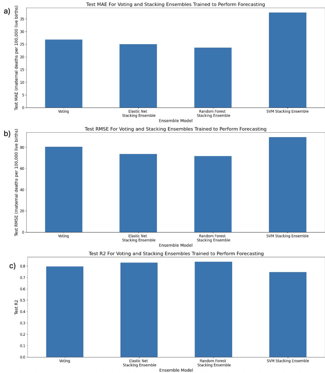
Figure A.10: a) Mean average error, b) root mean-squared error, and c) R^2 for voting and stacking ensembles trained on all base models to perform forecasting.
