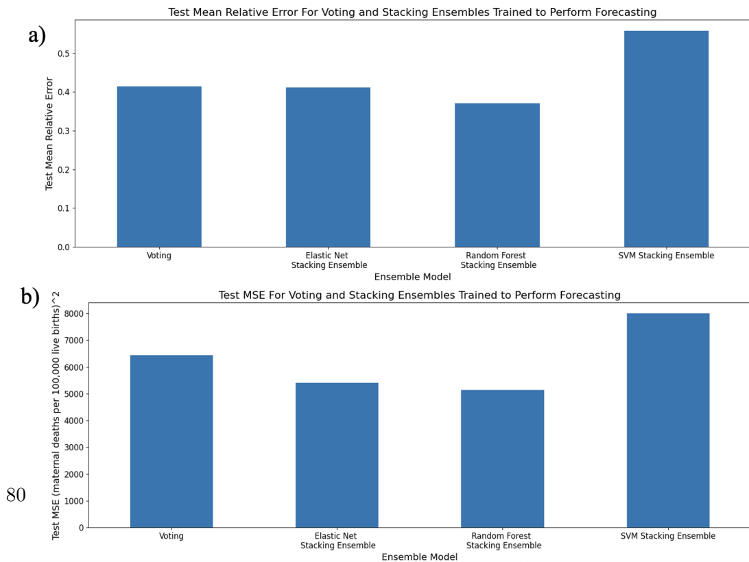
Figure 5.19: a) Mean relative error and b) mean-squared error for voting and stacking ensembles trained on all base models to perform forecasting.
