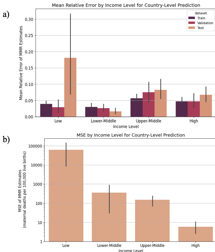
Figure 5.28: a) Mean relative error and b) mean-squared error (log scale) for income-level specific MMR estimates from the Random Forest Stacking Ensemble used for country-level prediction. MRE was given for its performance on the train, validation, and test sets. MSE was only given for the test set.
