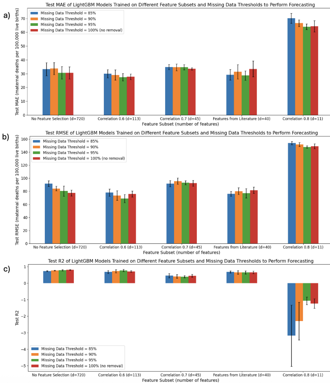
Figure A.6: a) Mean average error, b) root mean-squared error, and c) R^2 for LightGBM base estimators fit on different feature subsets and missing data thresholds to perform forecasting.
