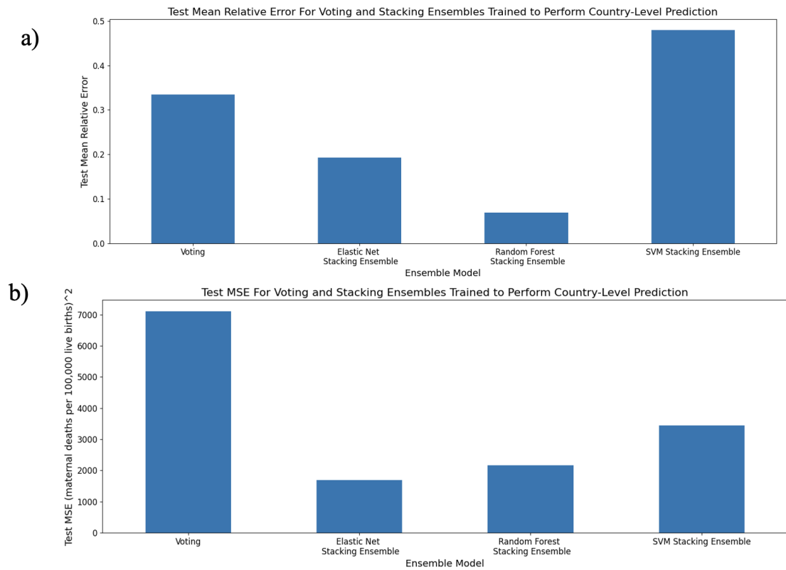
Figure 5.18: a) Mean relative error and b) mean-squared error for voting and stacking ensembles trained on all base models to perform country-level prediction.
