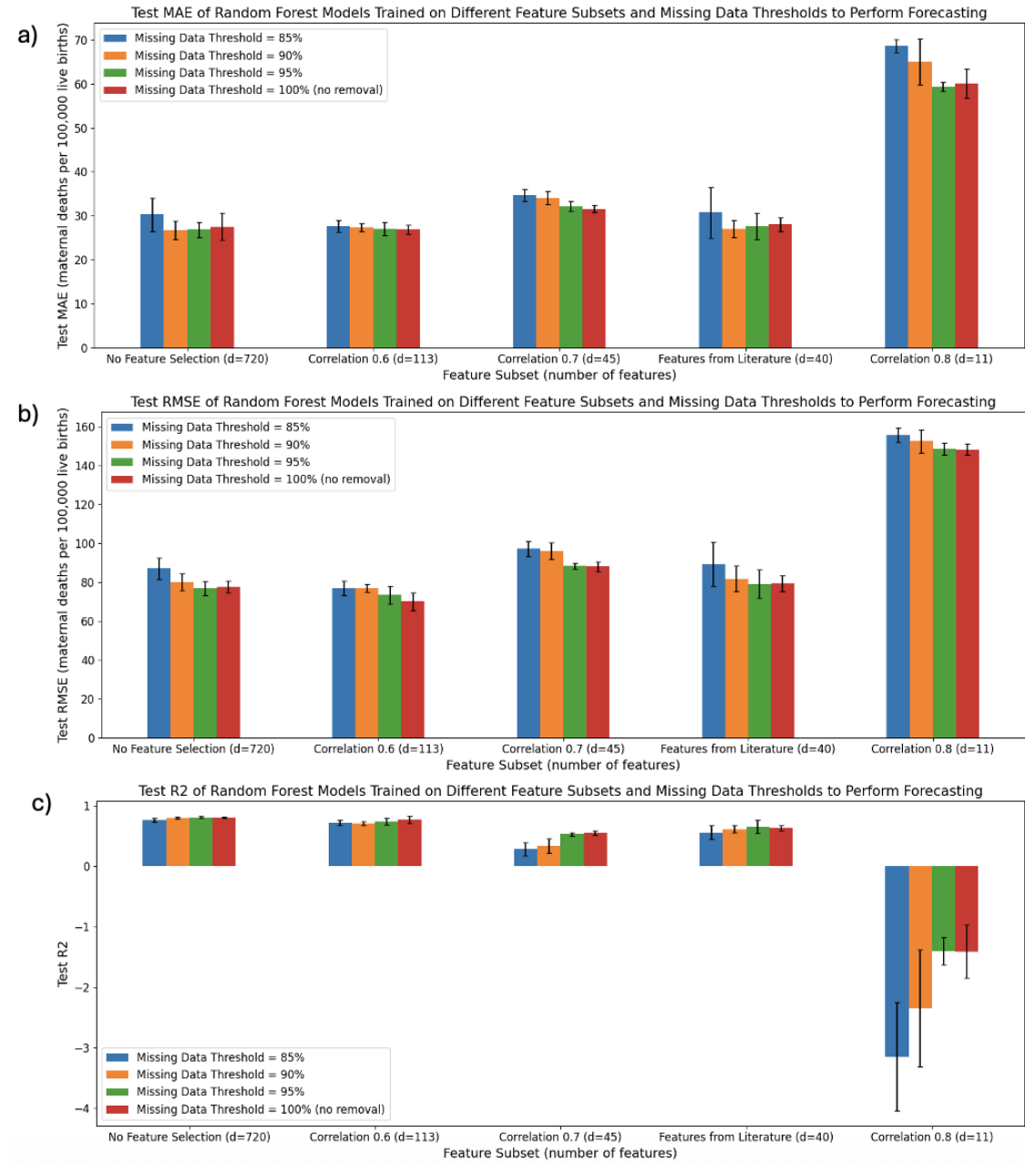
Figure A.4: a) Mean average error, b) root mean-squared error, and c) R^2 for Random Forest base estimators fit on different feature subsets and missing data thresholds to perform forecasting.
