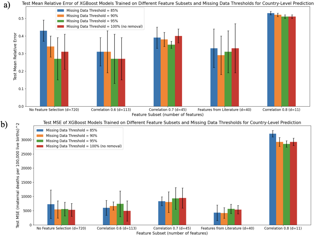
Figure 5.11: a) Mean relative error and b) mean-squared error for XGBoost base estimators fit on different feature subsets and missing data thresholds for country-level prediction.
