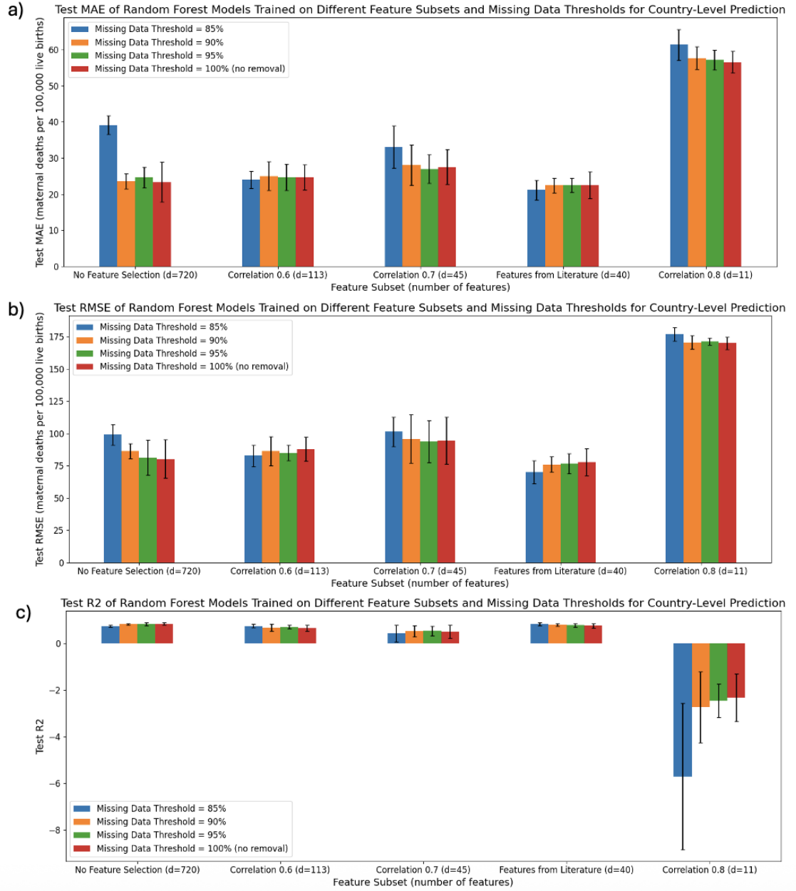
Figure A.1: a) Mean average error, b) root mean-squared error, and c) R^2 for Random Forest base estimators fit on different feature subsets and missing data thresholds for country-level prediction.
