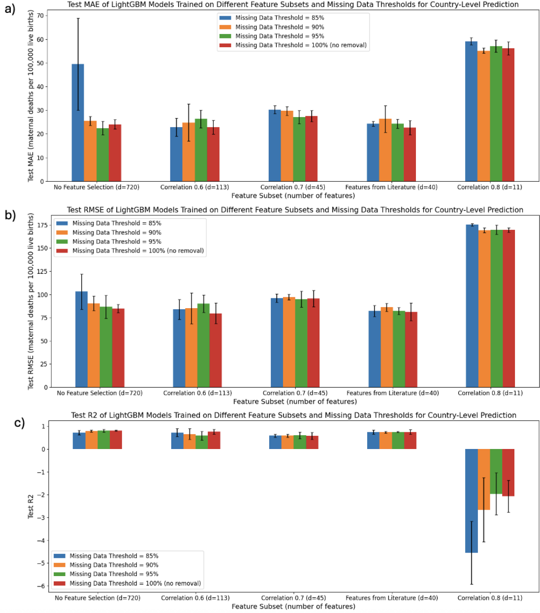
Figure A.3: a) Mean average error, b) root mean-squared error, and c) R^2 for LightGBM base estimators fit on different feature subsets and missing data thresholds for country-level prediction.
