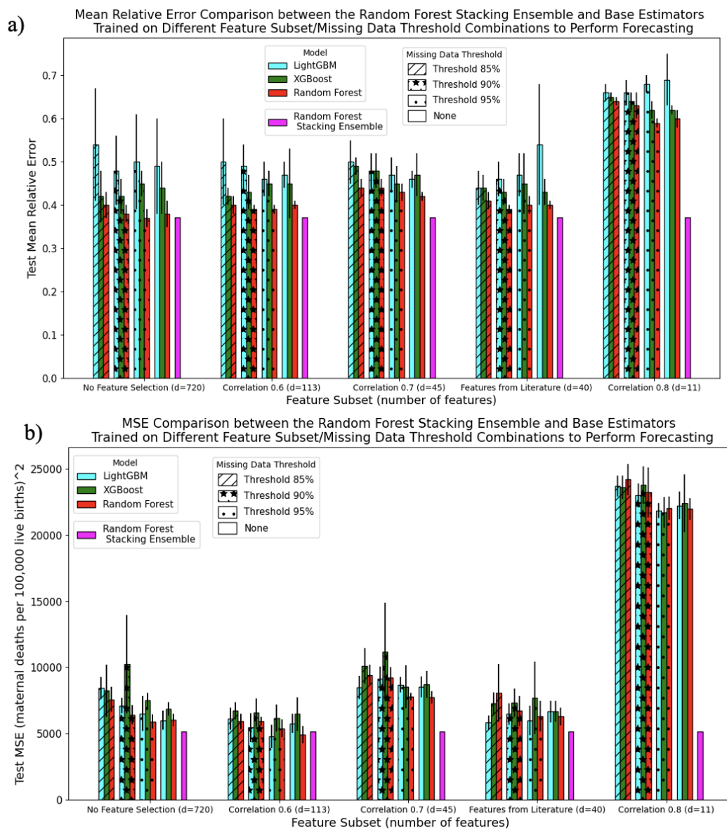
Figure 5.24: a) Mean relative error and b) mean-squared error of the Random Forest Stacking Ensemble (purple) and the Random Forest (red), XGBoost (green), and LightGBM (blue) base estimators trained for forecasting.
