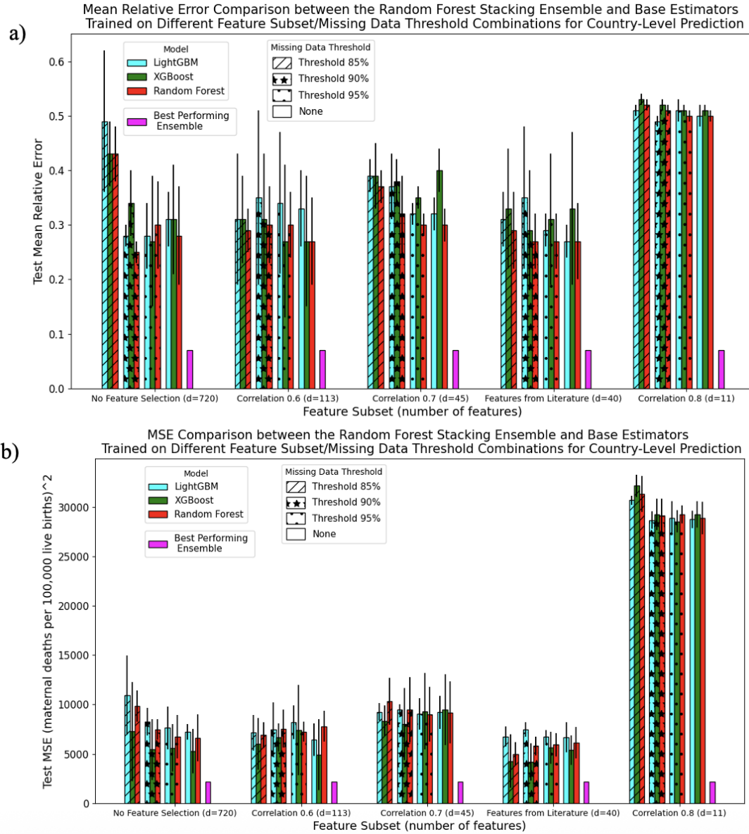
Figure 5.23: a) Mean relative error and b) mean-squared error for the Random Forest Stacking Ensemble (purple) and the Random Forest (red), XGBoost (green), and LightGBM (blue) base estimators trained for country-level prediction.
