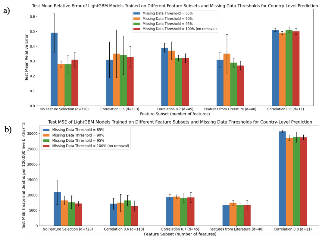
Figure 5.12: a) Mean relative error and b) mean-squared error for LightGBM base estimators fit on different feature subsets and missing data thresholds for country-level prediction.
