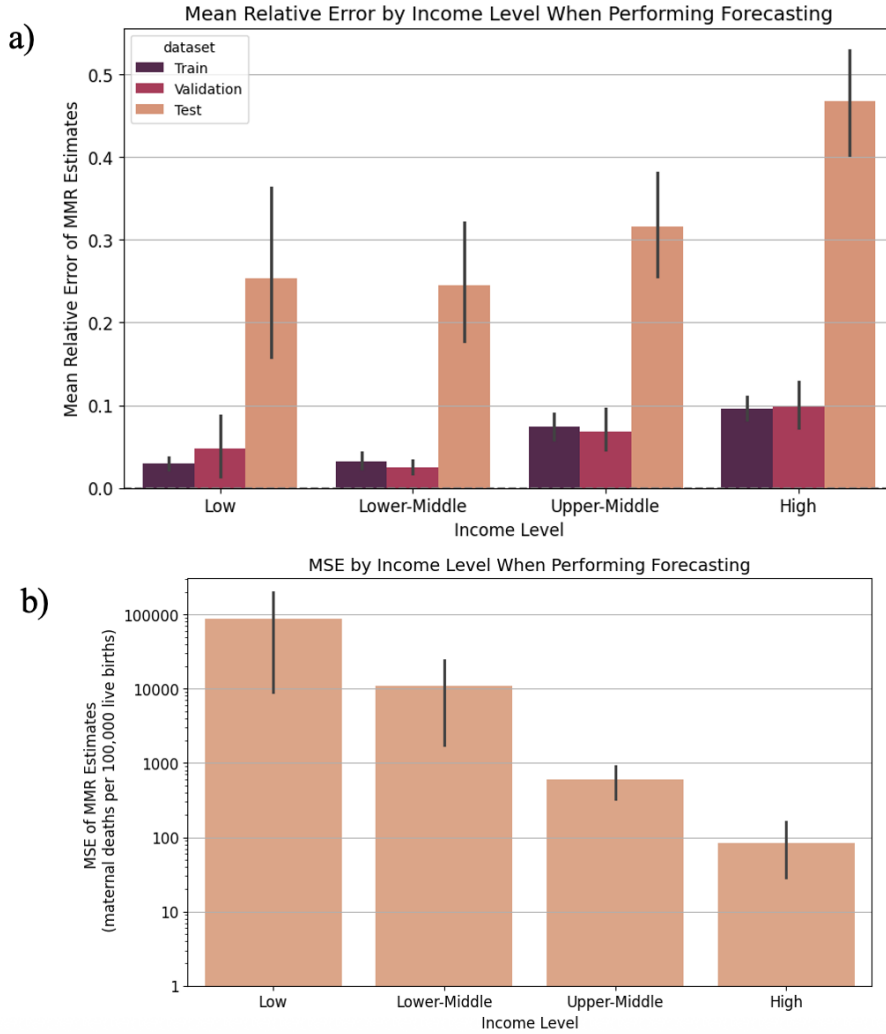
Figure 5.29: a) Mean relative error and b) mean-squared error (log-scale) for income-level specific MMR predictions from the Random Forest Stacking Ensemble trained to perform forecasting. MRE was given for the RFSE's performance on the train, validation, and test sets. MSE was only given for the test set.
