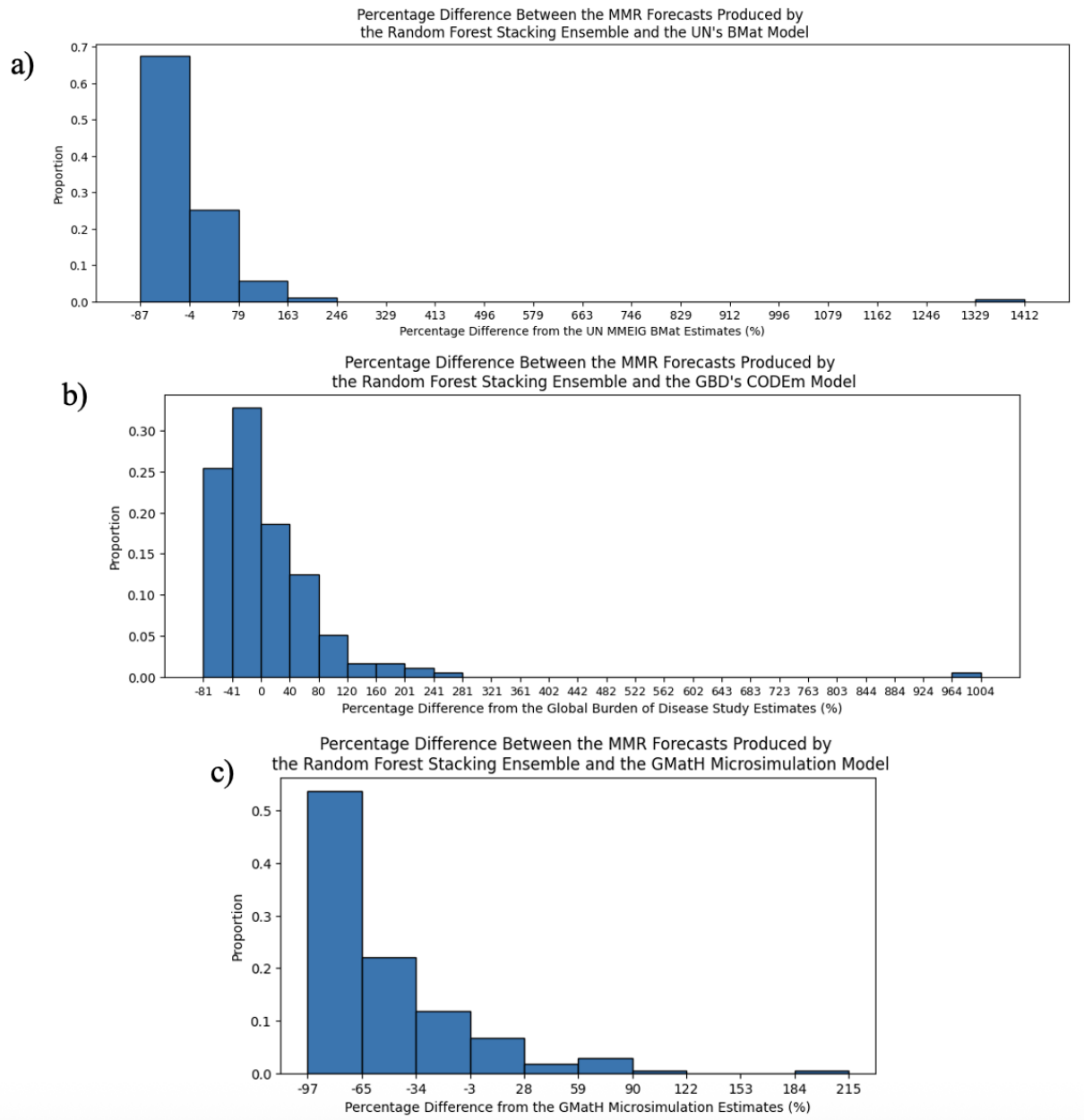
Figure 5.34: Percentage difference between MMR estimated by my best-performing Random Forest Stacking Ensemble trained to perform forecasting and the MMR estimated by a) BMat b) CODEm, and c) GMatH.
