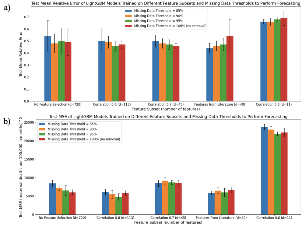
Figure 5.15: a) Mean relative error and b) mean-squared error for LightGBM base estimators fit on different feature subsets and missing data thresholds for forecasting.
